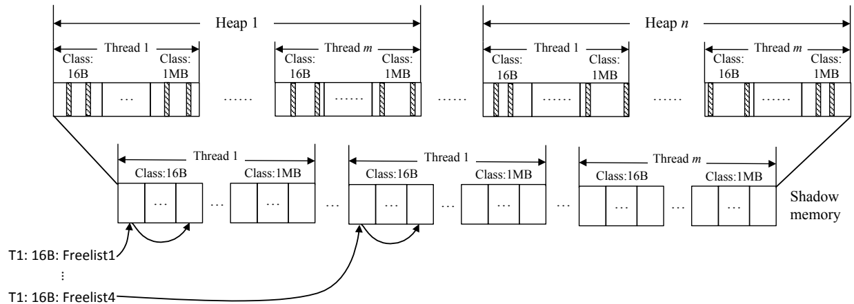
Figure 3: One example of FreeGuard's layout.
