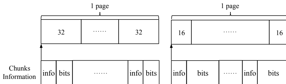
Figure 2: A fragment of the OpenBSD allocator. The mapping between bags and metadata (e.g. chunks information) is kept in a global hash table, and each bag has a bitmap to maintain the status of all objects inside. Metadata are typically stored in a separate location.
